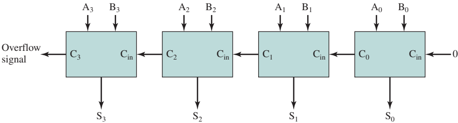
Figure 11.19 4-Bit Adder
