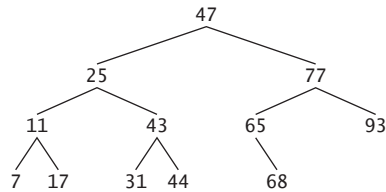
Fig. 22.16 | Binary search tree containing 12 values.
