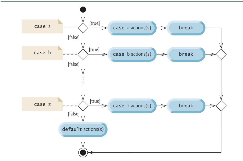
Fig. 5.11 | switch multiple-selection statement UML activity diagram with break statements.
