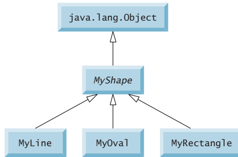
Fig. 10.17 | MyShape hierarchy.
